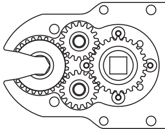
GEAR ASSEMBLY
