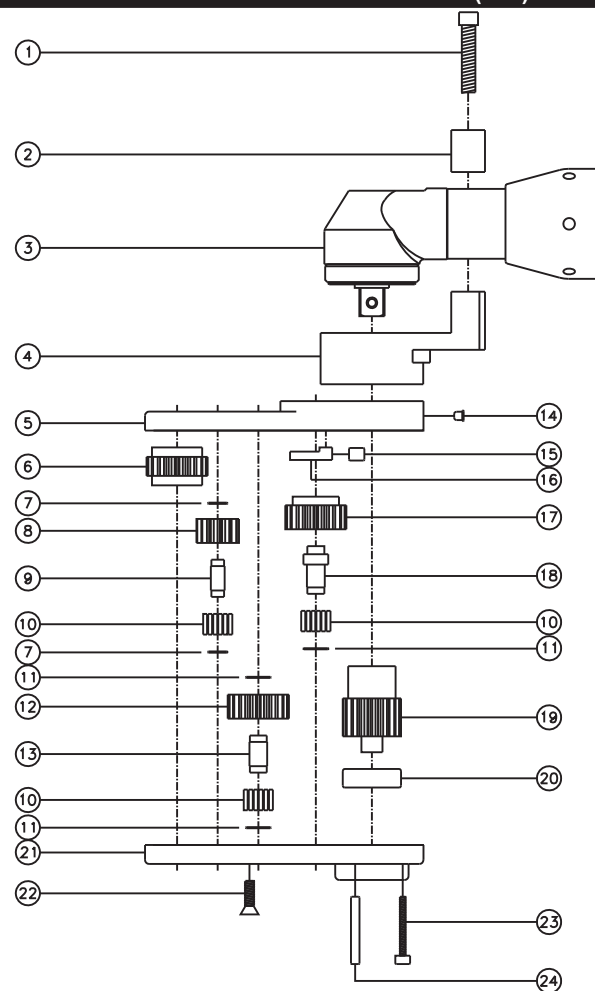
PARTS BLOWOUT
